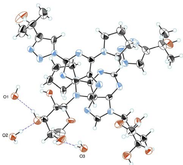
Fig. 3. A view of asymmetric unit of the compound 10 ·H 2 O
